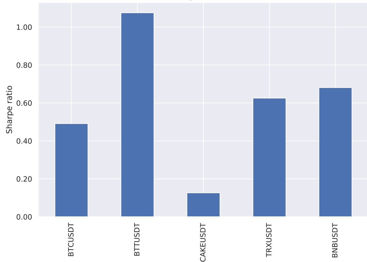
Sharpe (Details)
