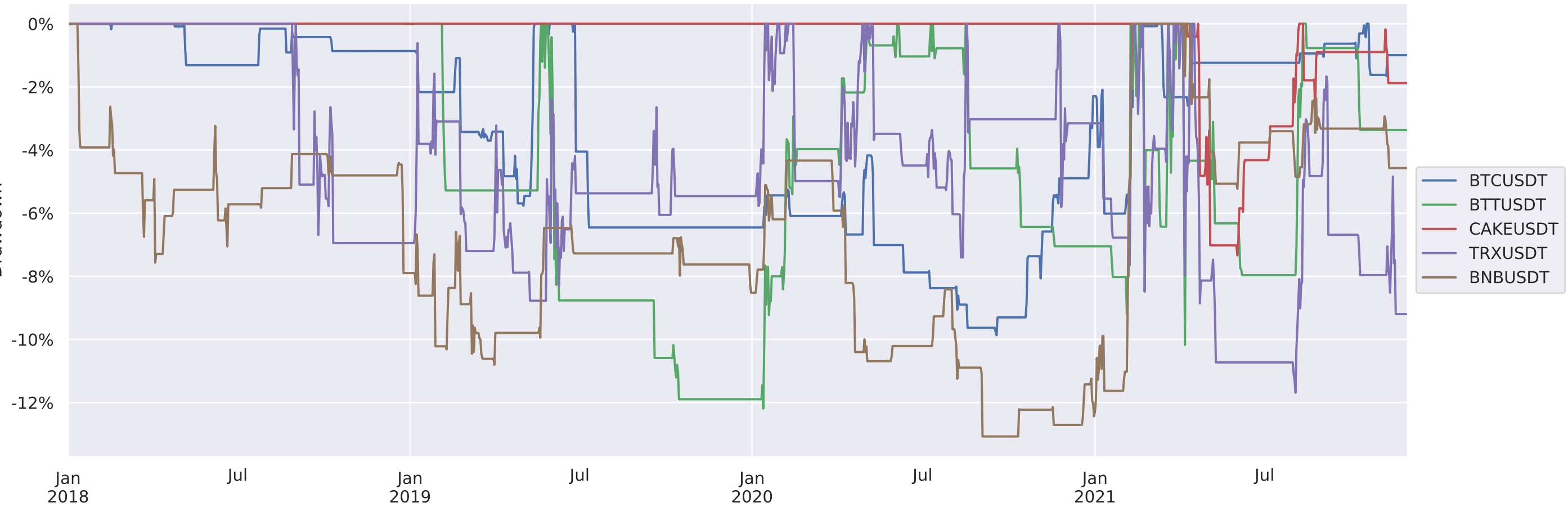
Drawdowns (Details)
